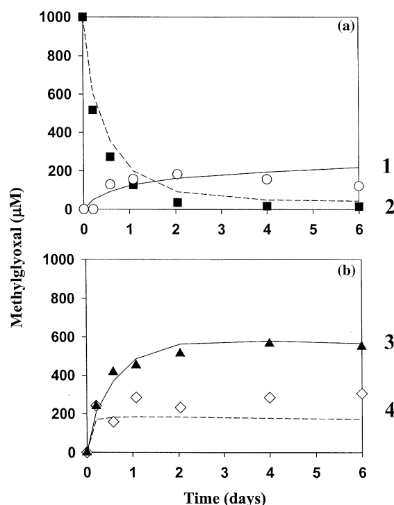
Figure 3. Model predictions for reaction of methylglyoxal (1 mM) with BSA (100 \mu M) at physiological pH and temperature. Data (symbols) were obtained from Lo et al. (1994) and are compared with Model #1 predictions (lines) for reaction of MG in this system. For modeling purposes, BSA is treated as a pool of free arginine, lysine and cysteine at concentrations of 2300 \mu M, 6100 \mu M and 300 \mu M, respectively. (a) Degraded MG (1) and free MG (2); (b) irreversibly bound MG (3) and reversibly bound MG (4).
